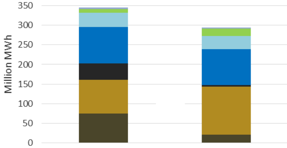
Total generation mix in RGGI states
